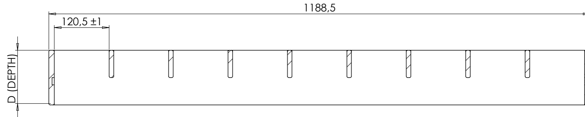
SECTION B-B
