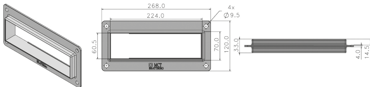
Frame Article no: CS00001800
