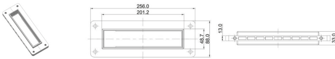
Frame Article no: RFCS001600
