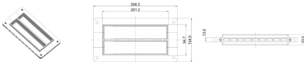
Frame Article no: RFCS003200
