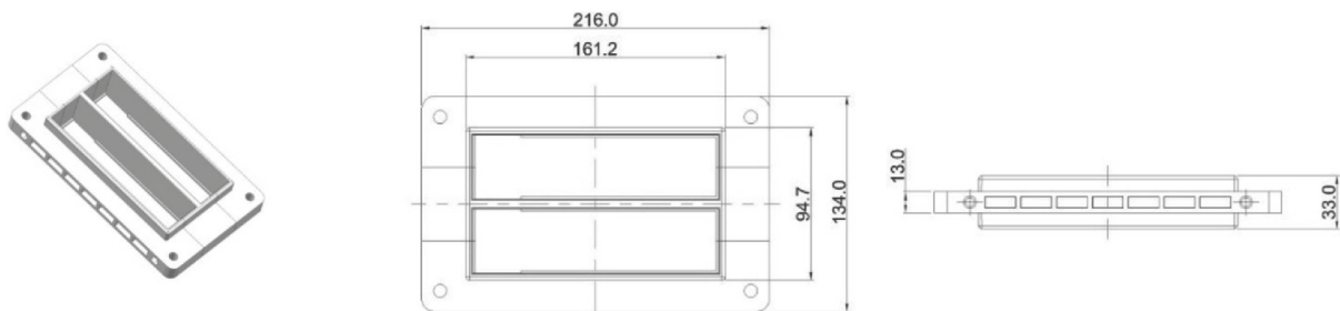
Frame Article no: RFCS002400
